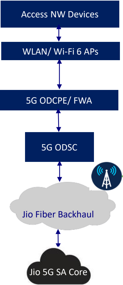
5G as a fallback option to SD-WAN network over MPLS
